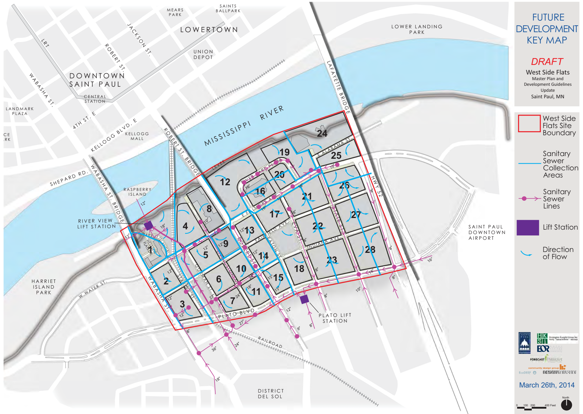
Figure 2: Existing Sanitary Sewer Infrastructure Network
