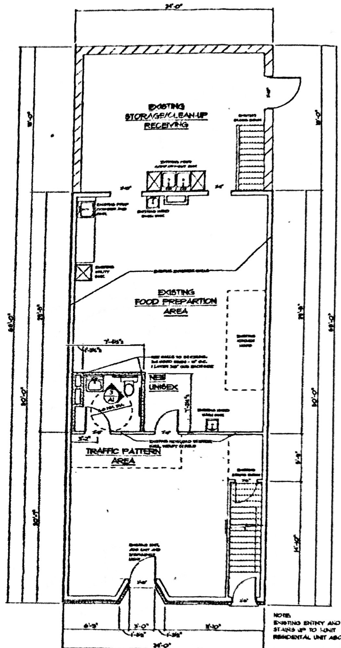
① FIRST FLOOR PLAN
