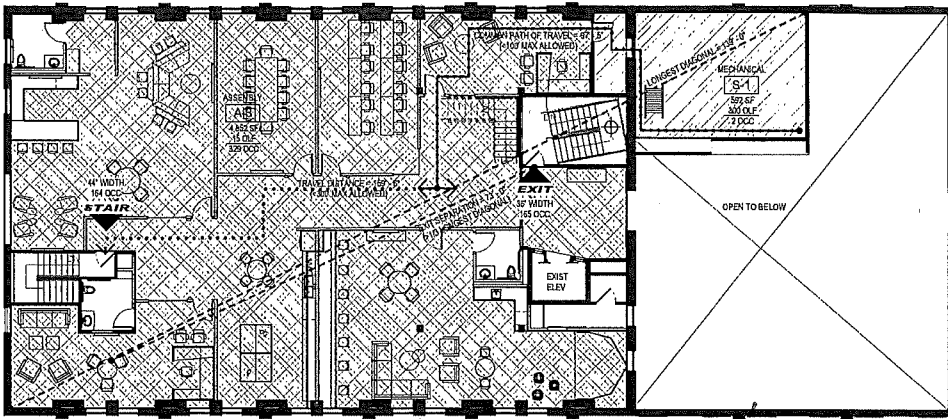
3 LIFE SAFETY PLAN - LEVEL 02 3/32" = 1'-0"
