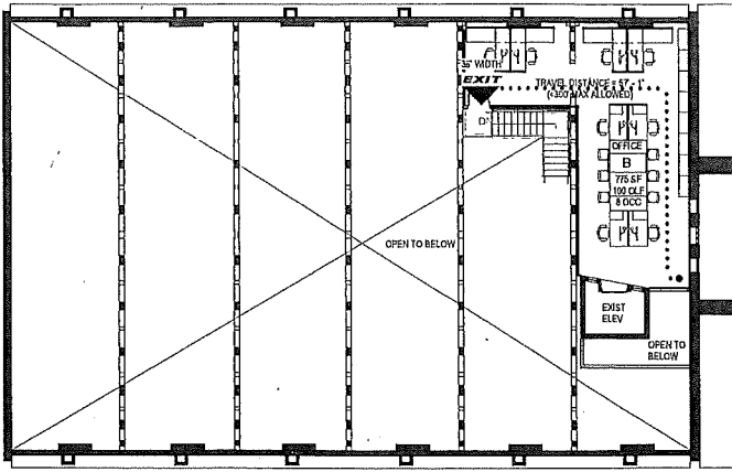
4 MEZZANINE - LEVEL 03 3/32" = 1'-0"
