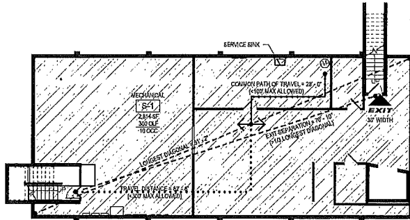
2 LIFE SAFETY PLAN - LOWER LEVEL 3/32" = 1'-0"
