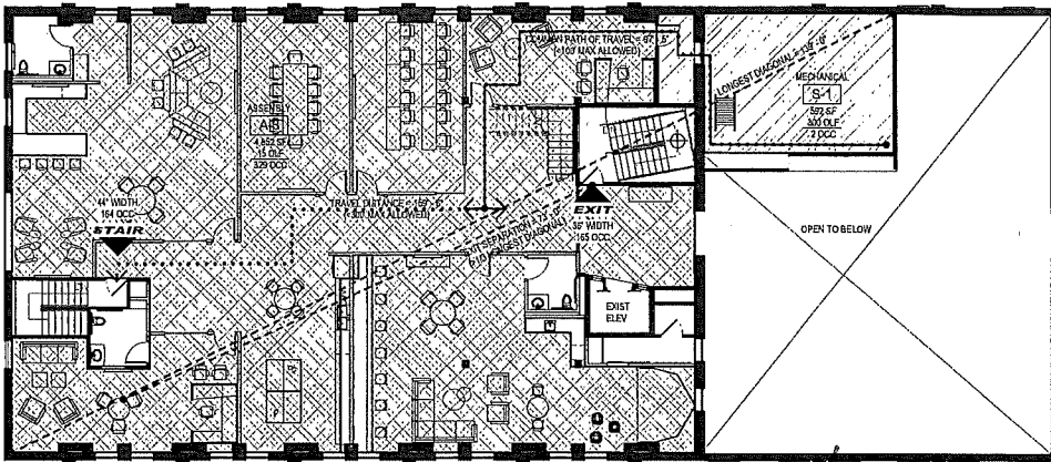
3 LIFE SAFETY PLAN - LEVEL 02 3/32" = 1/4"
