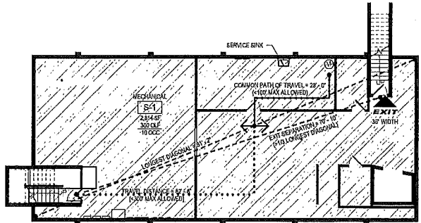
2 LIFE SAFETY PLAN - LOWER LEVEL 3/32" = 1/4"
