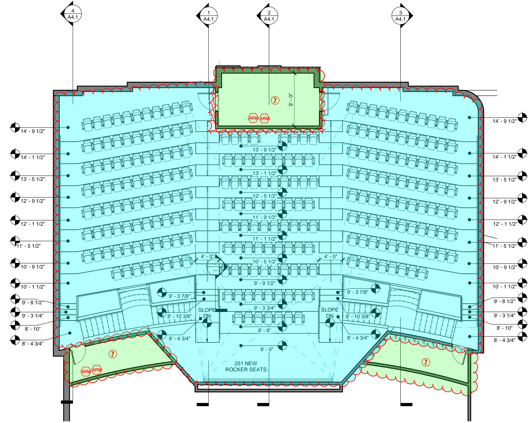
2 SECOND FLOOR PLAN A2.1 SCALE: 1/8" = 1'-0"
