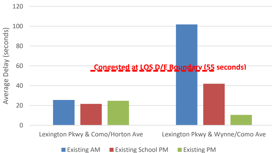
Chart 1 – Peak Hour Delays: Signal Controlled Intersections
