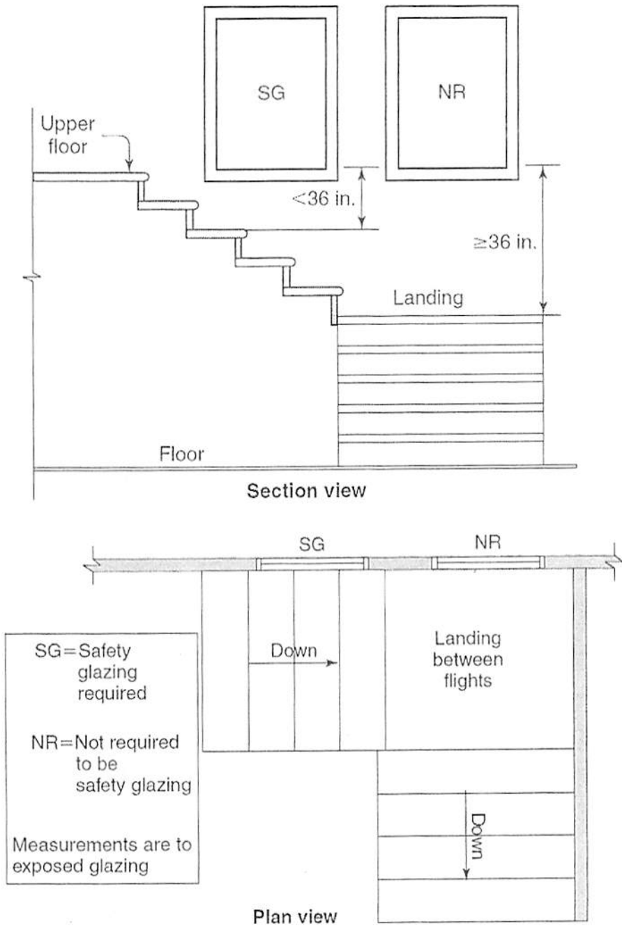
Figure 9: Glazing adjacent stairs and landings between flights of stairs
