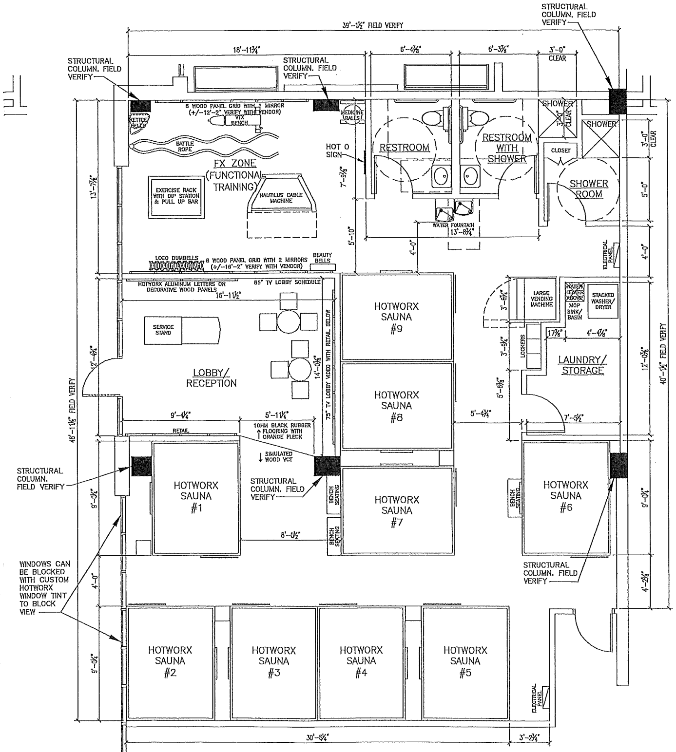
PROPOSED FLOORPLAN SCALE 1/4" = 1'-0"
