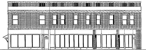
② South Elevation 1/8" = 1'-0"
