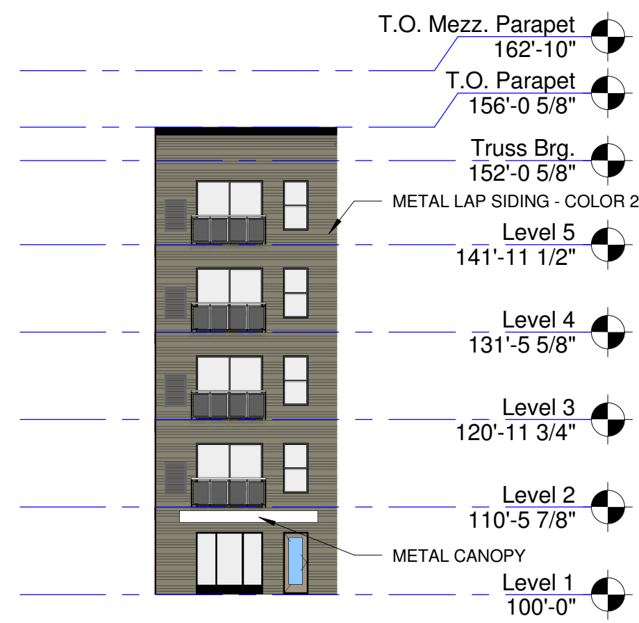
② CY Elevation 2 Marketing 1/16" = 1'-0"
