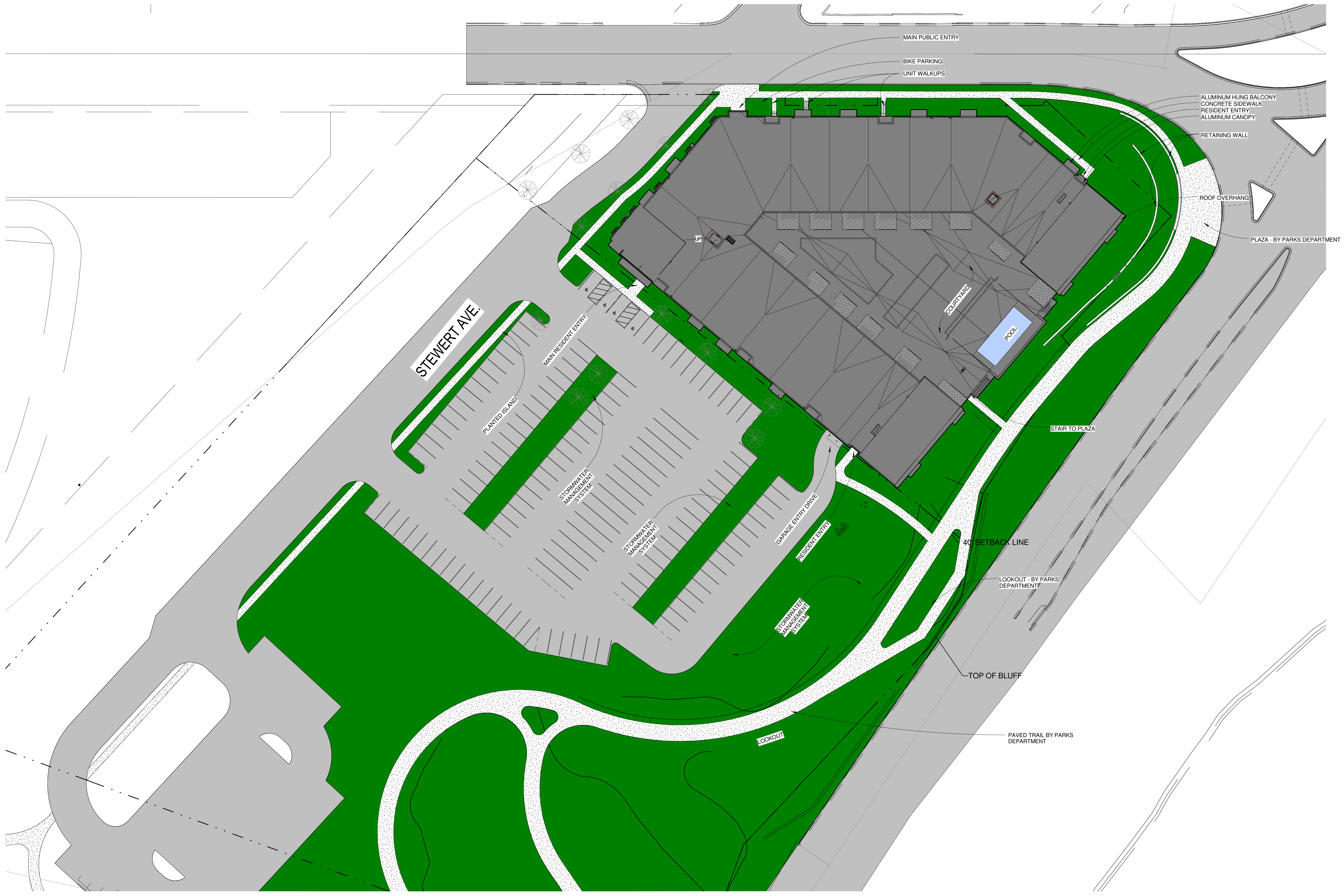
1 Site Plan 1/32" = 1'-0"
