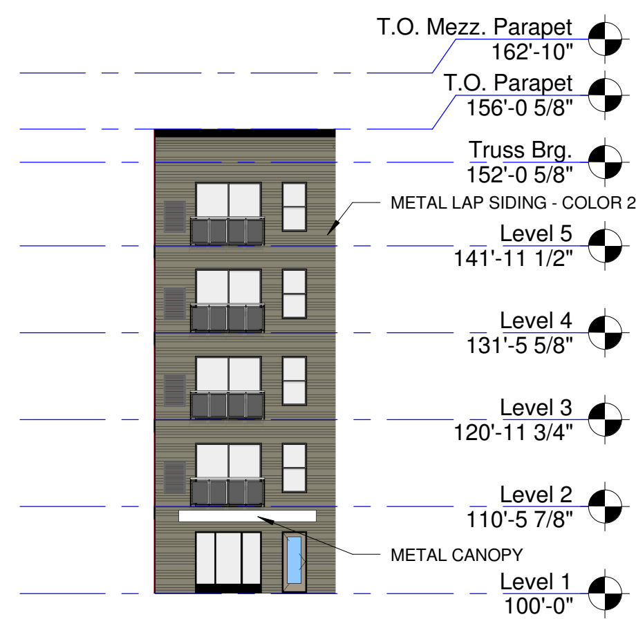
2 CY Elevation 2 Marketing 1/16" = 1'-0"
