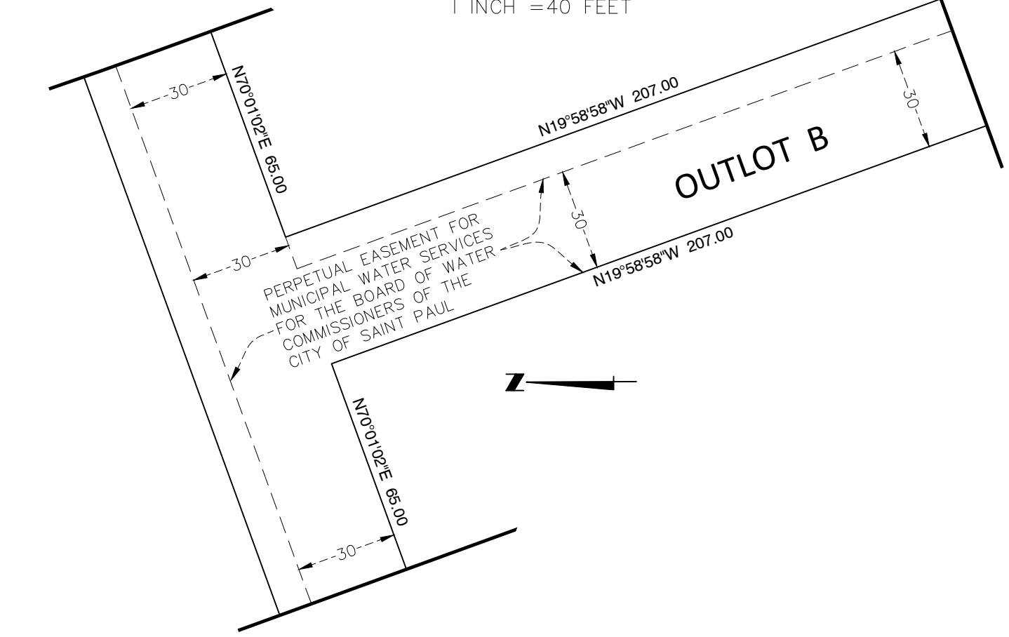
EASEMENT DETAIL 1 INCH = 40 FEET
