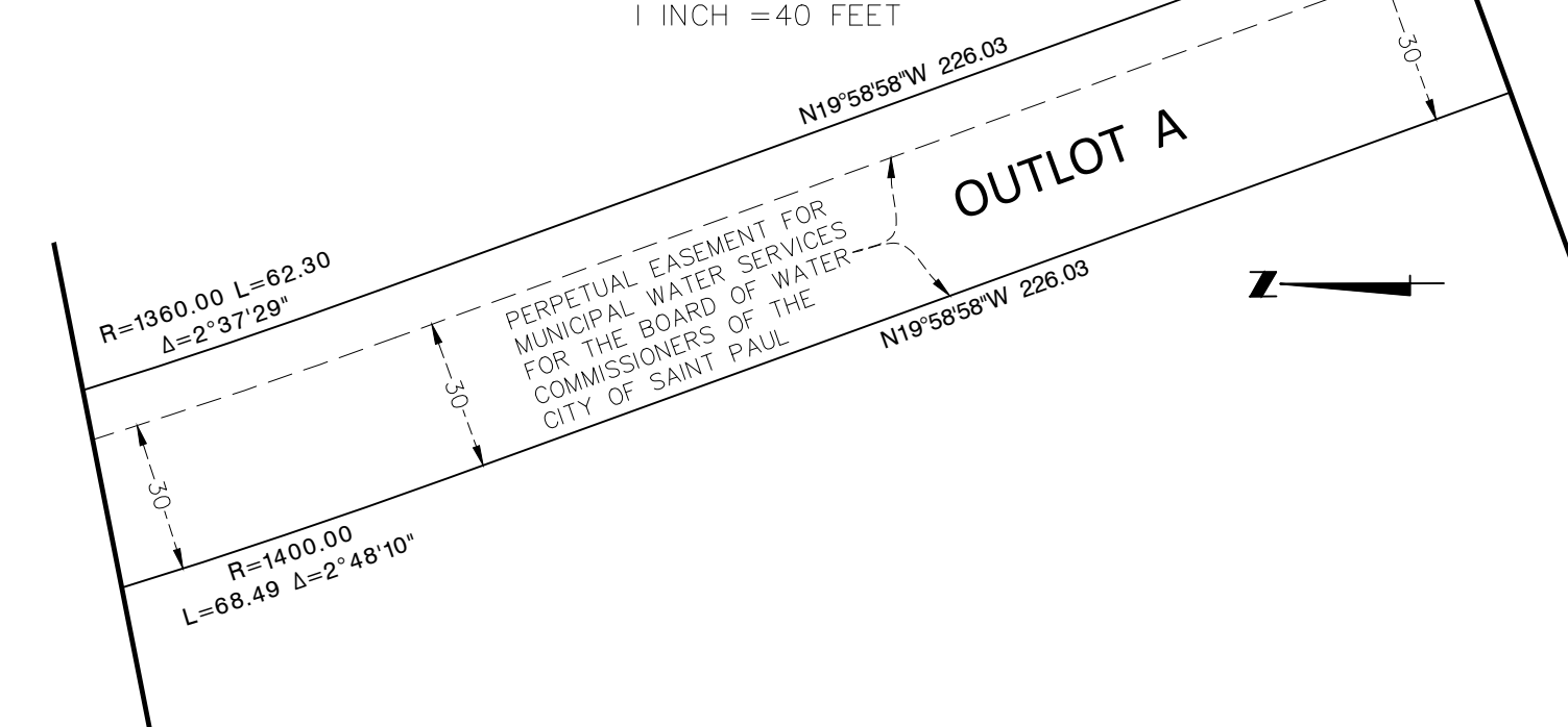
EASEMENT DETAIL 1 INCH = 40 FEET
