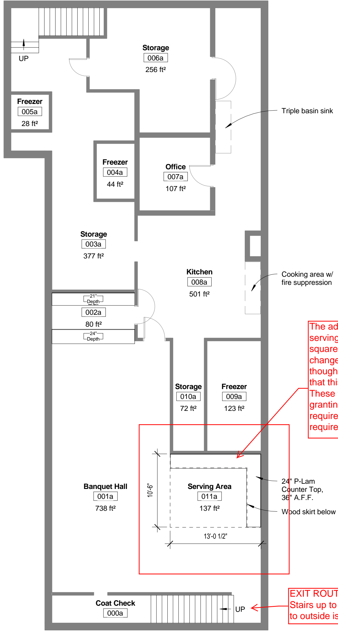
① Level -1 Option A 1/8" = 1'-0"
