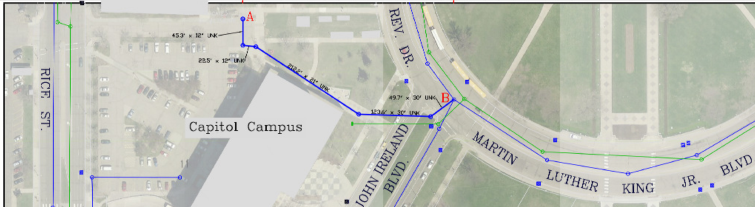
CAPITOL CAMPUS STORM PIPES
