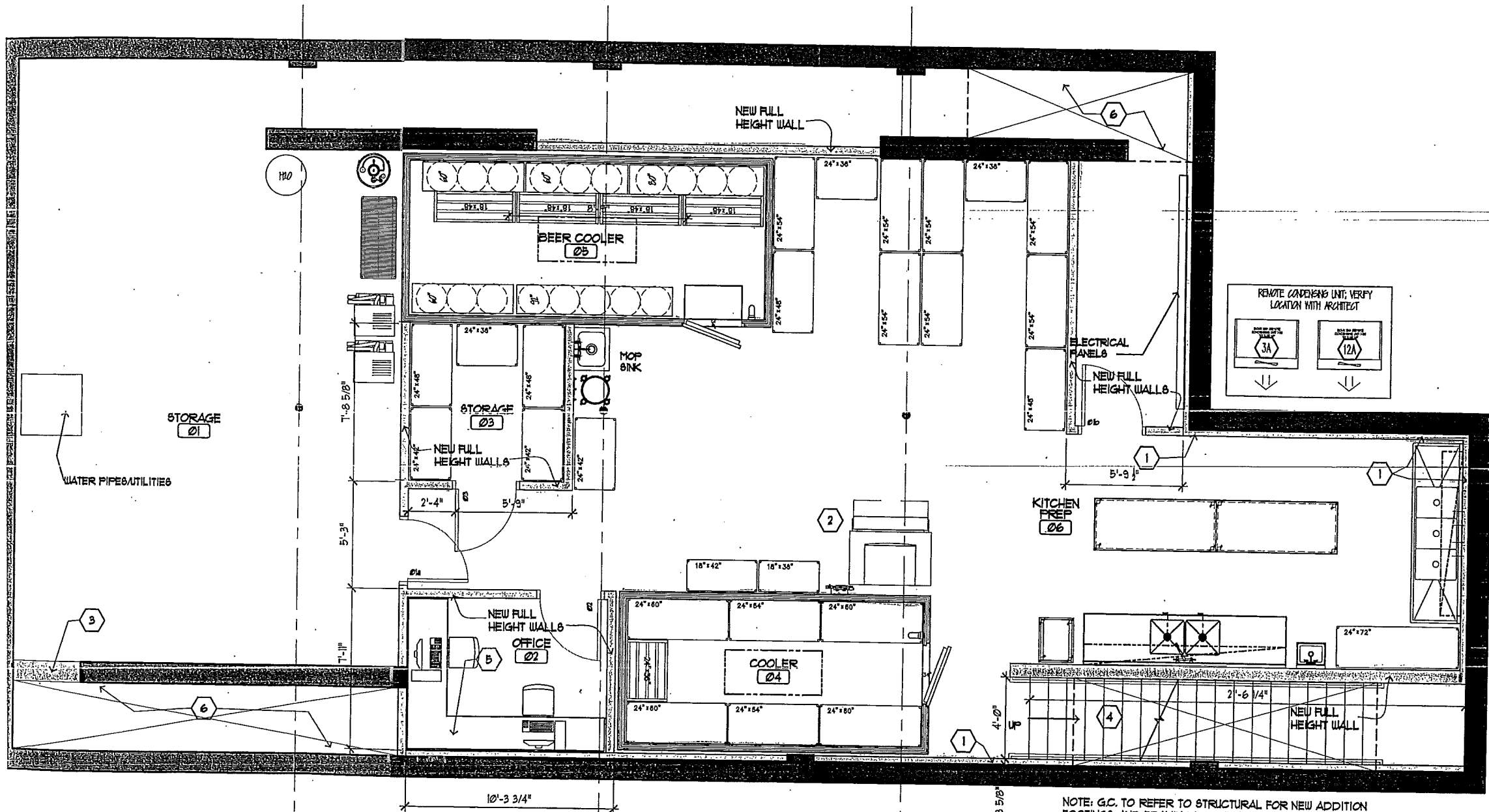
BASEMENT ARCHITECTURAL PLAN 1/8" = 1'-0"
