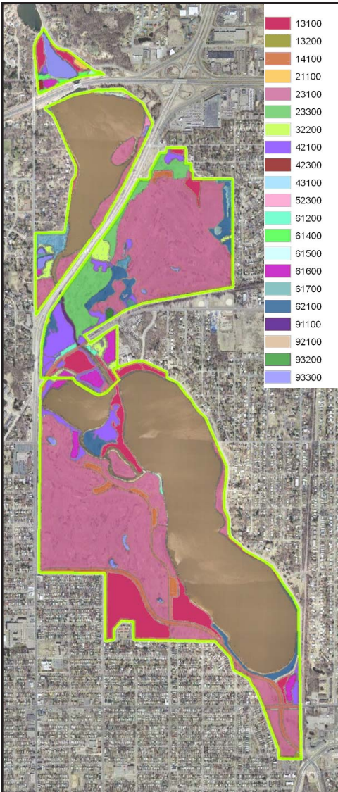
FIGURE 11.2 - MLCCS Coverages
