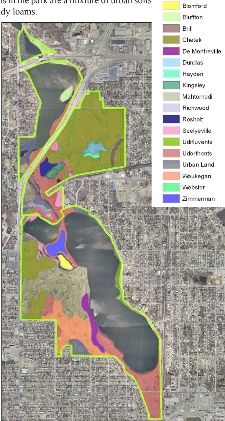
FIGURE 11.5 - Soils
