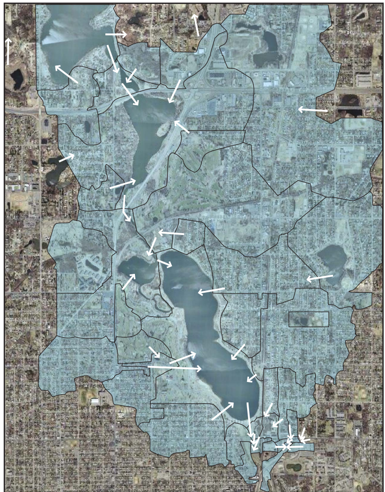
FIGURE 11.4 - Watershed
