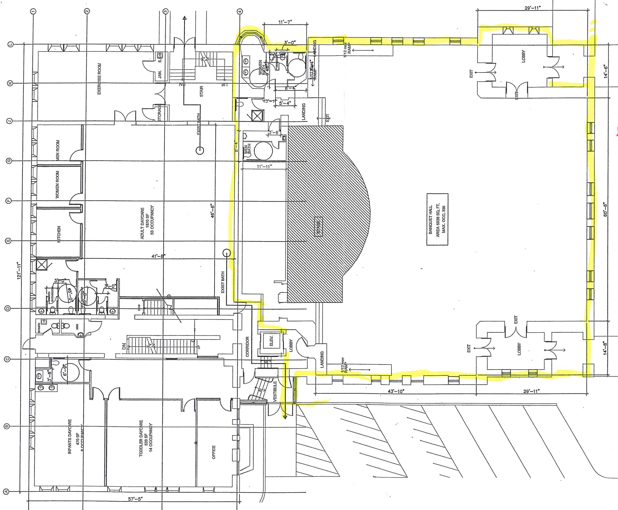
1 FIRST FLOOR PLAN (FULL) A5.0 1/16"=1'-0"
