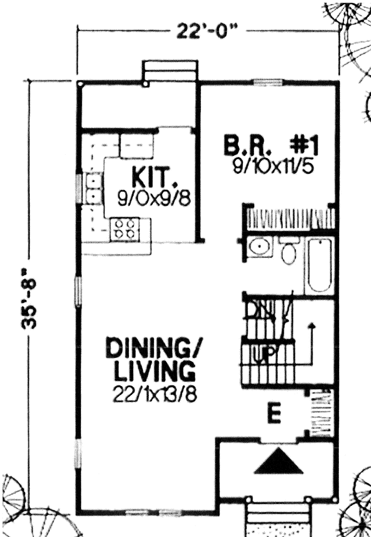
Home Plan: LS-1083-HDG Second Floor Plan
