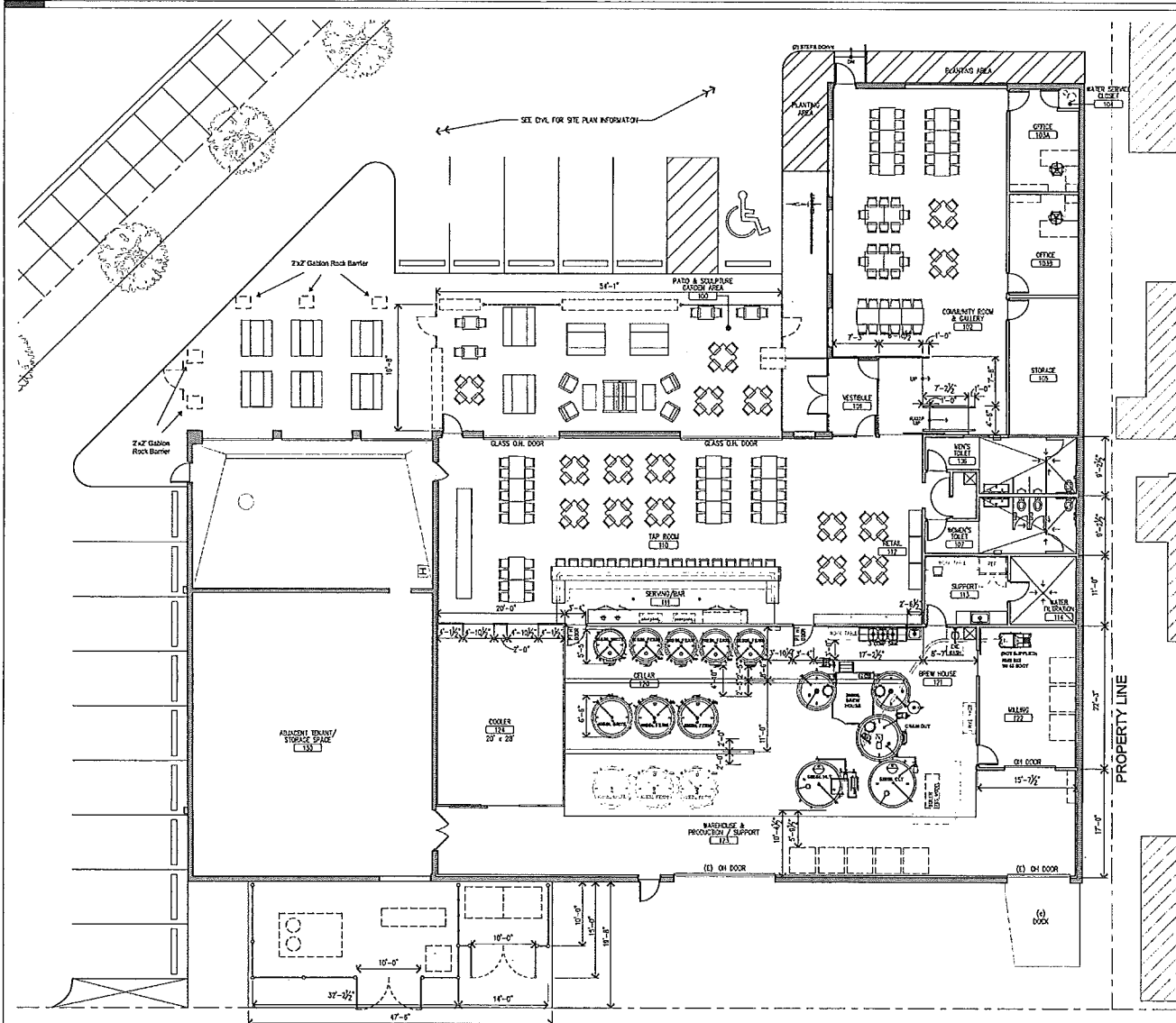
1 FLOOR PLAN 1/8" = 1'-0"
