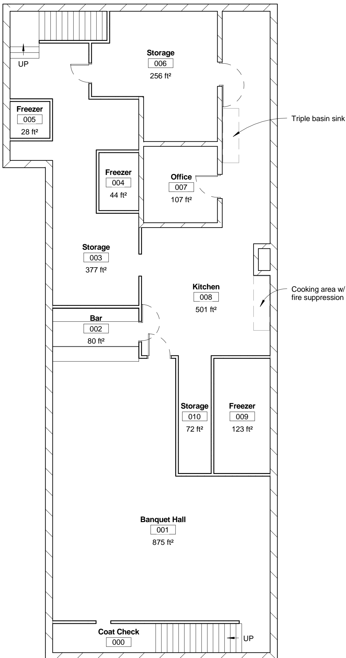
1 Level -1 1/8" = 1'-0"
