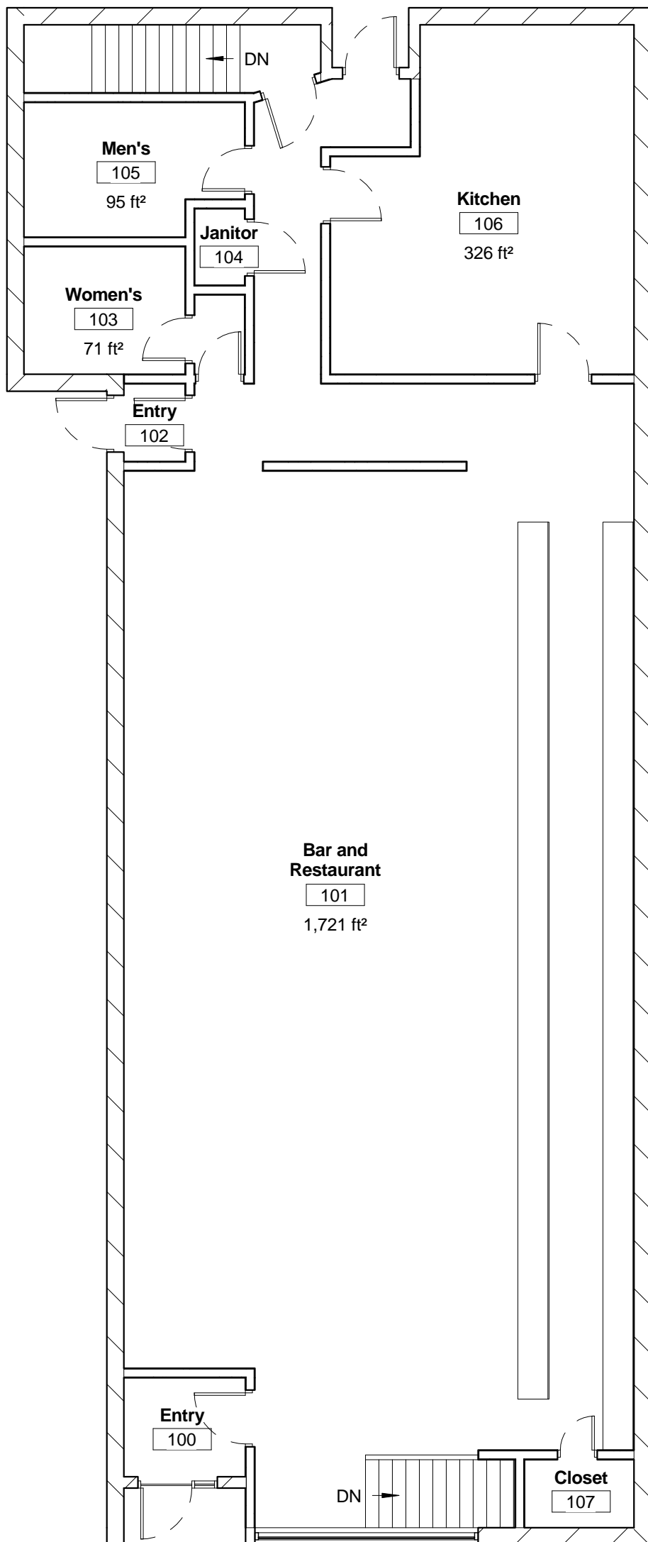
① Level 1 1/8" = 1'-0"
