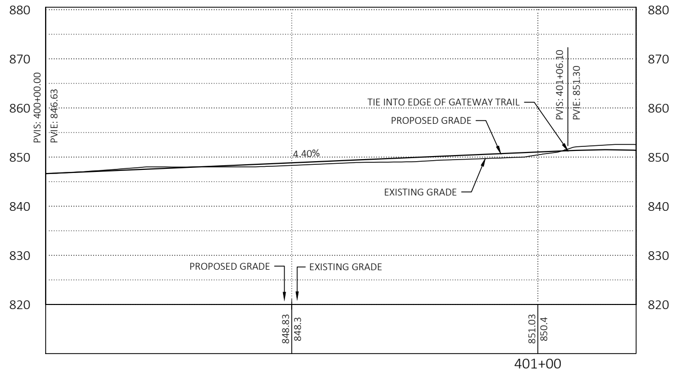
2 Profile View
