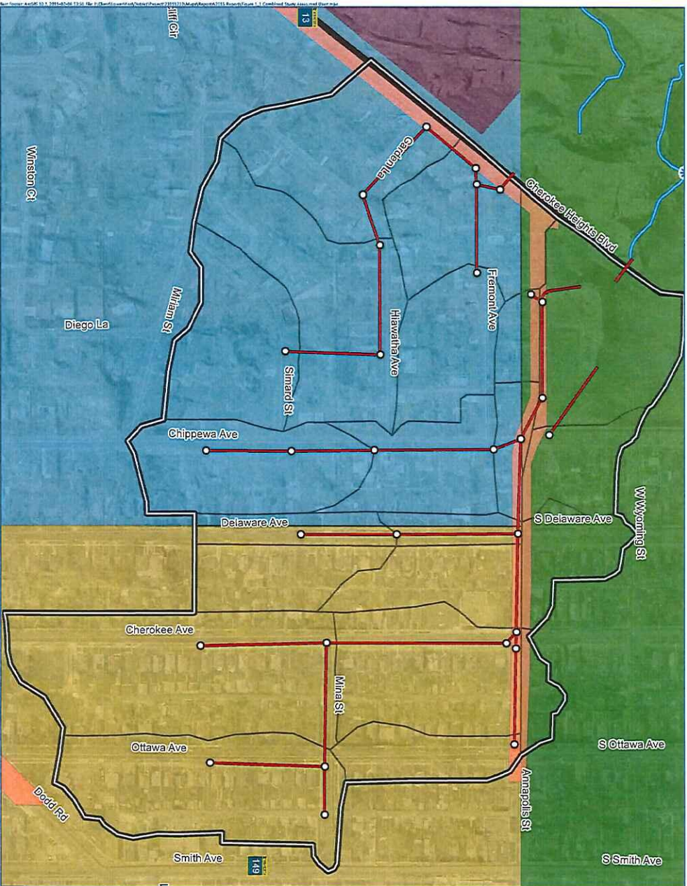
CONTRIBUTING AREAS CHEROKEE HEIGHTS' CLVERT ANALYSIS AND EROSION CONTROL FEASIBILITY STUDY Figure 6-1
