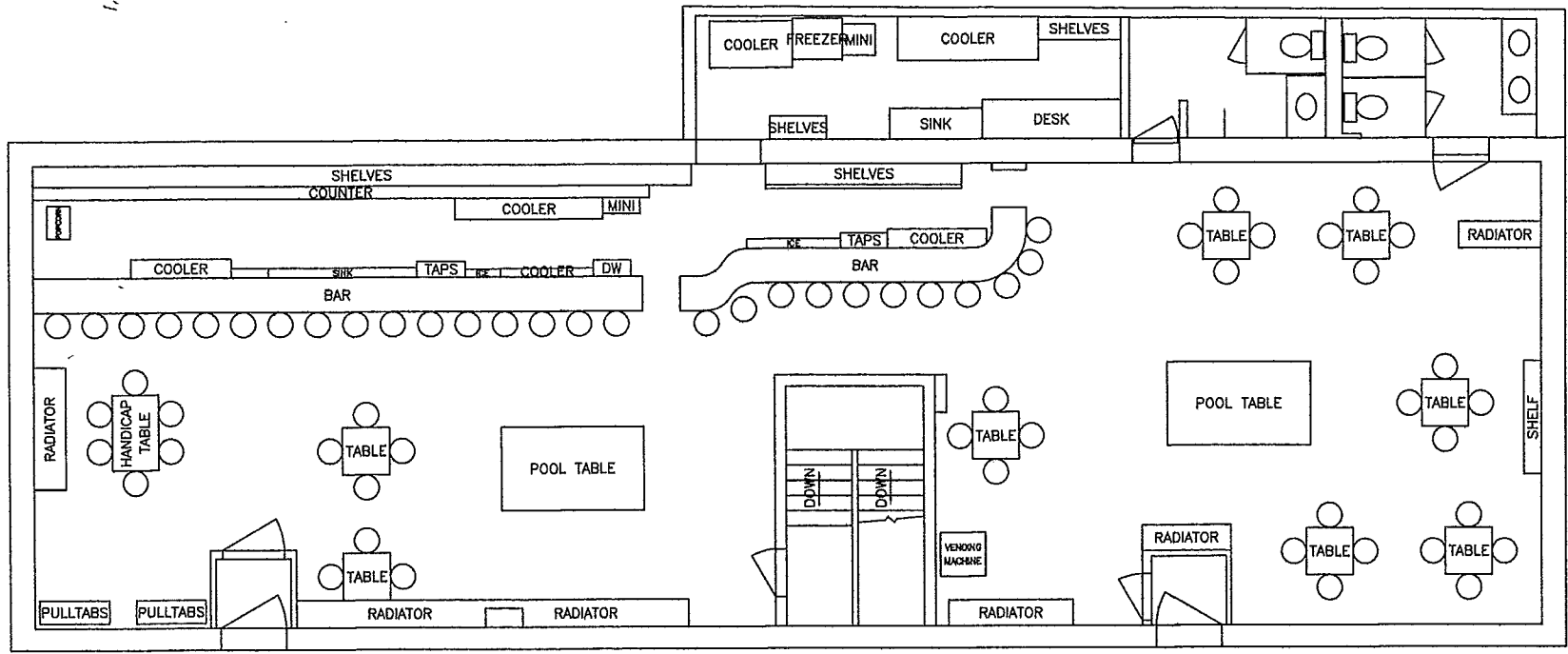
MAIN LEVEL PLAN VIEW
