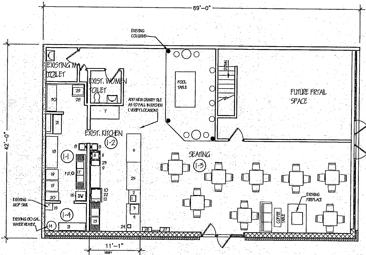
FLOOR PLAN
