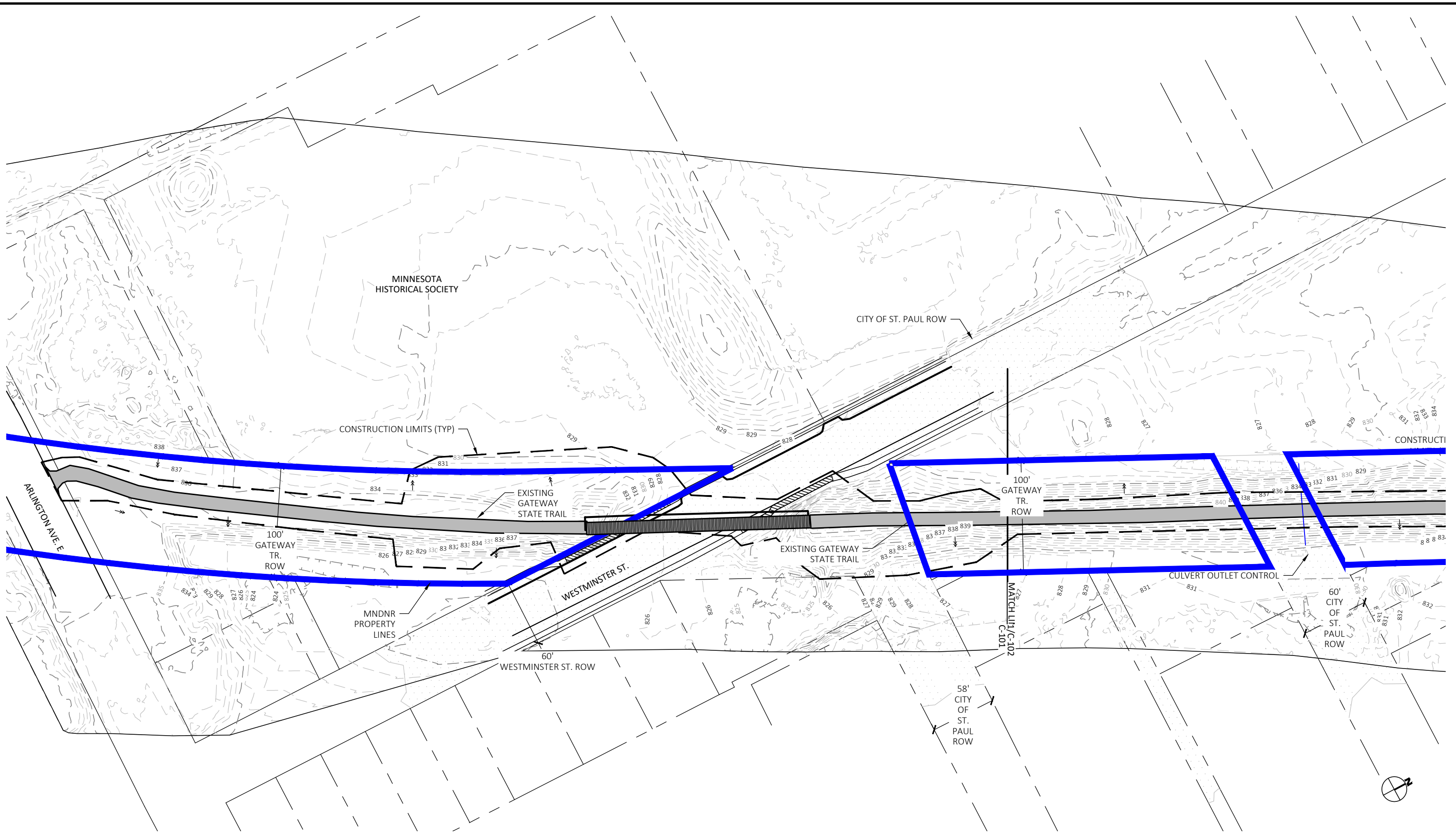
1 SITE PLAN - EXHIBIT A - DNR PROPERTY LINES
