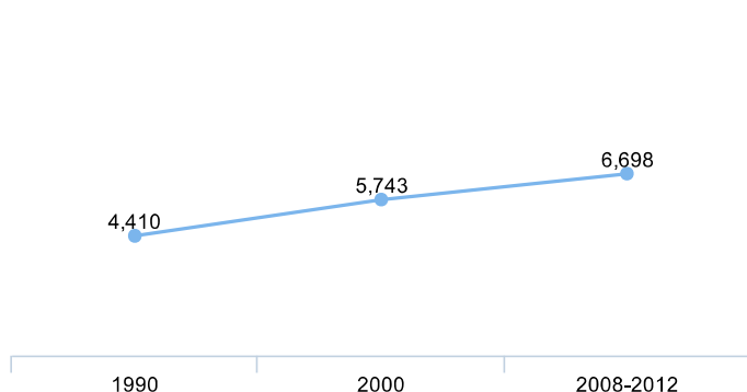
Total population
