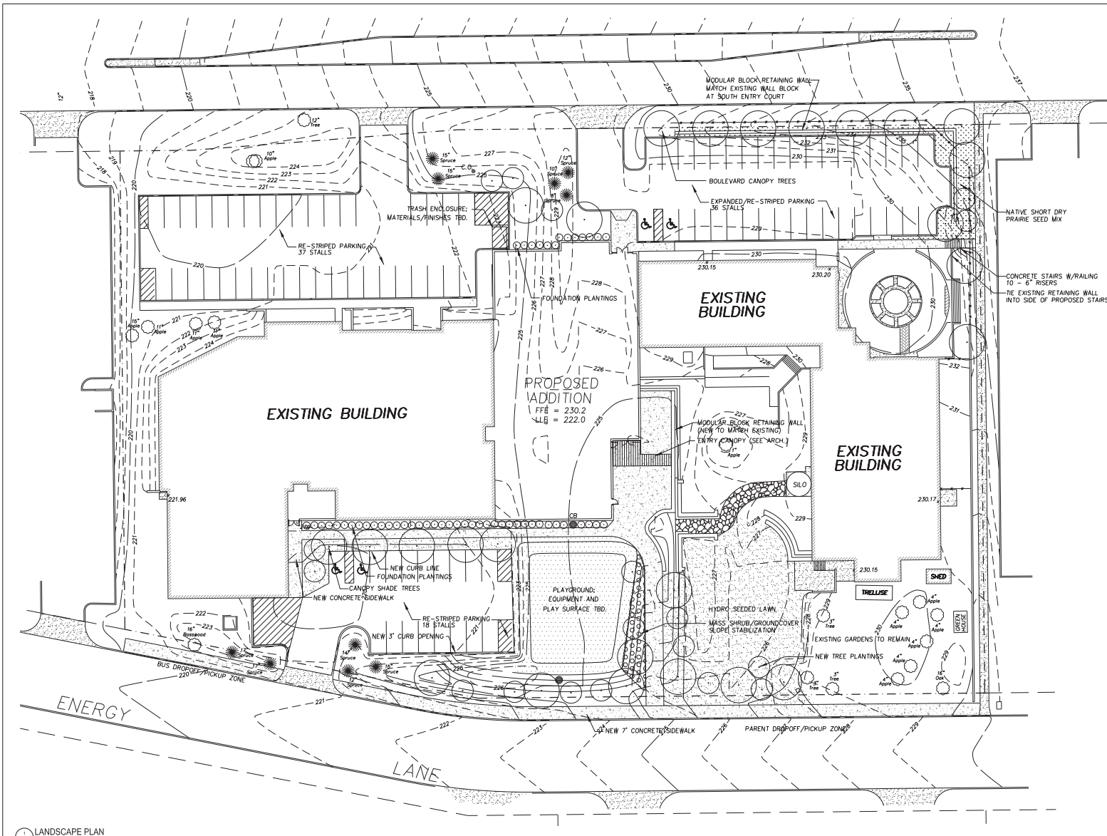
LANDSCAPE PLAN 1" = 20' 0" 0' 10' 20'
