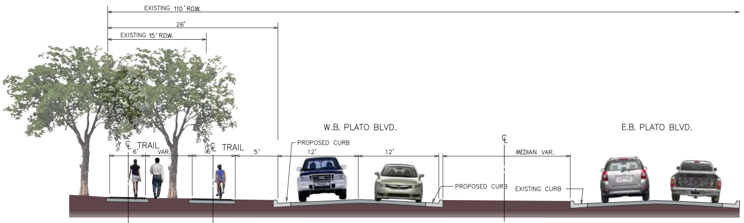
PLATO BOULVD. SECTION TYPE #1
