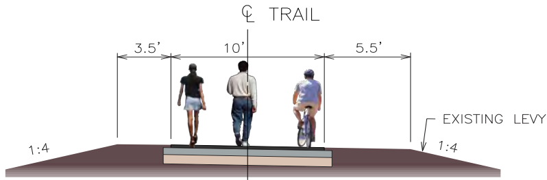
LEVEE SECTION
