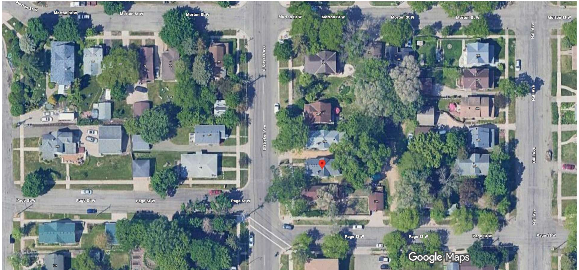
Imagery ©2026 Airbus, CNES / Airbus, Maxar Technologies, Map data ©2026 Google 20 ft
