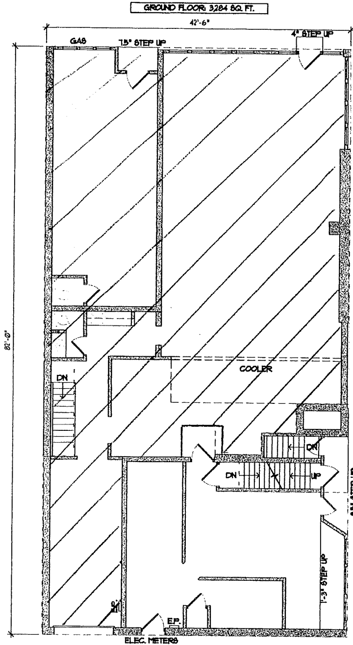
1 GROUND FLOOR PLAN A-1 1/8" = 1'-0"
